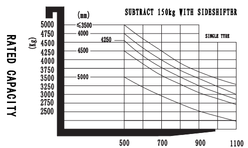
CPD50F8 LOAD CENTRE POSITION (mm)
