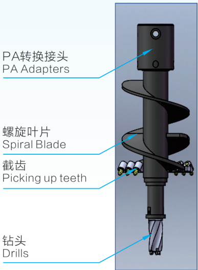
全叶片钻杆 All-Vane Drill Pipe
